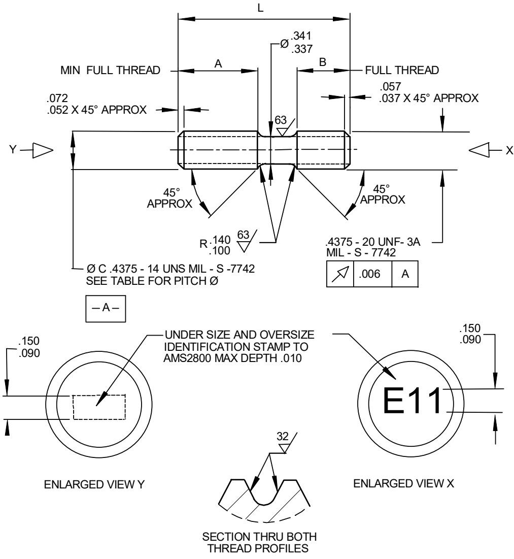
FIGURE 1 - STUD
